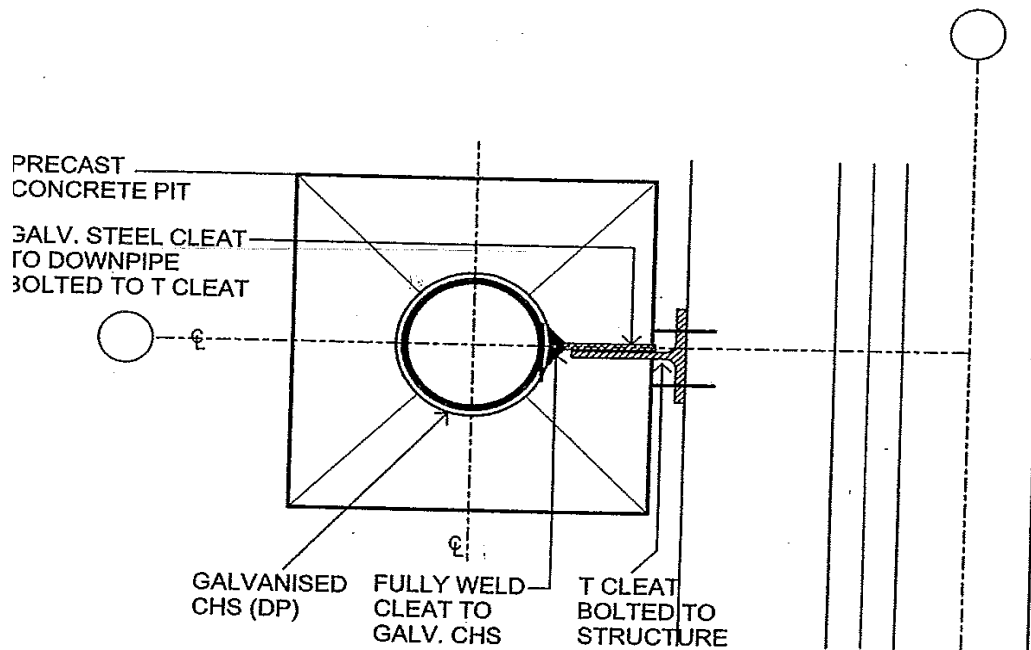
TYPICAL DOWNPIPE SUMP DETAIL 1:5
