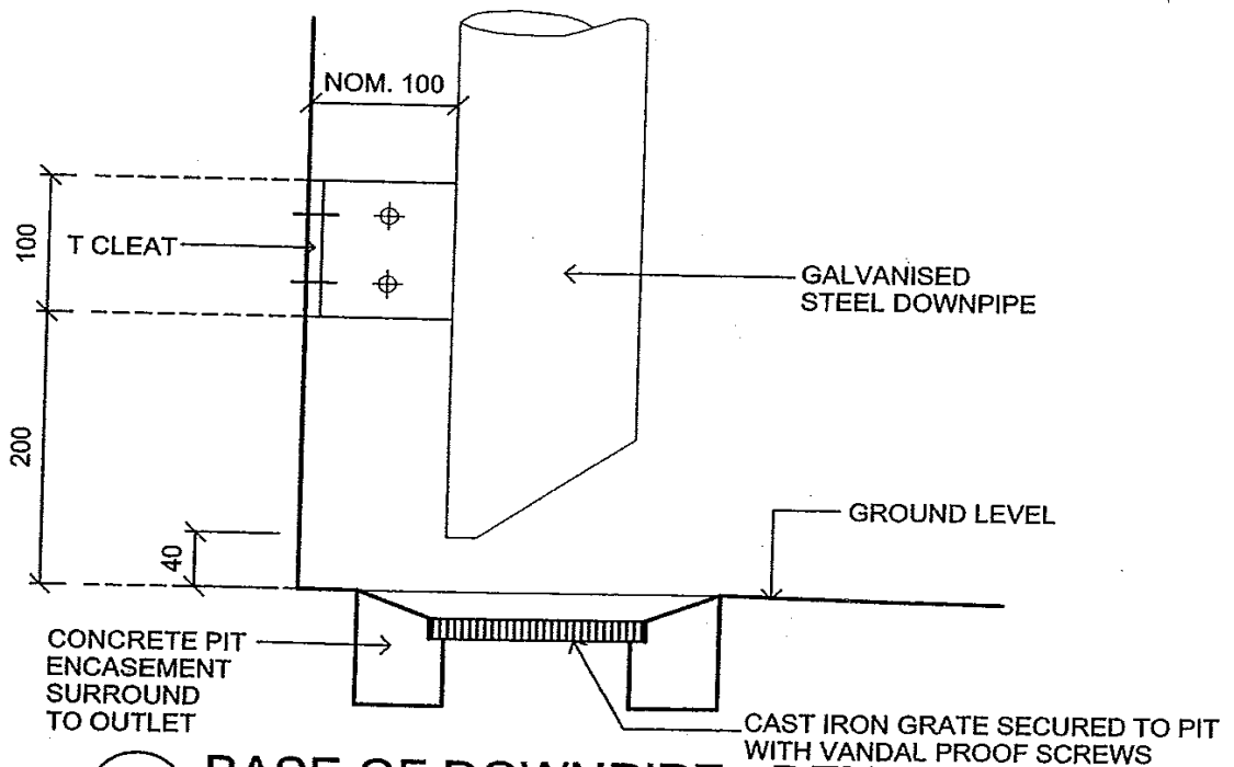
BASE OF DOWNPIPE - DETAIL 1:5
